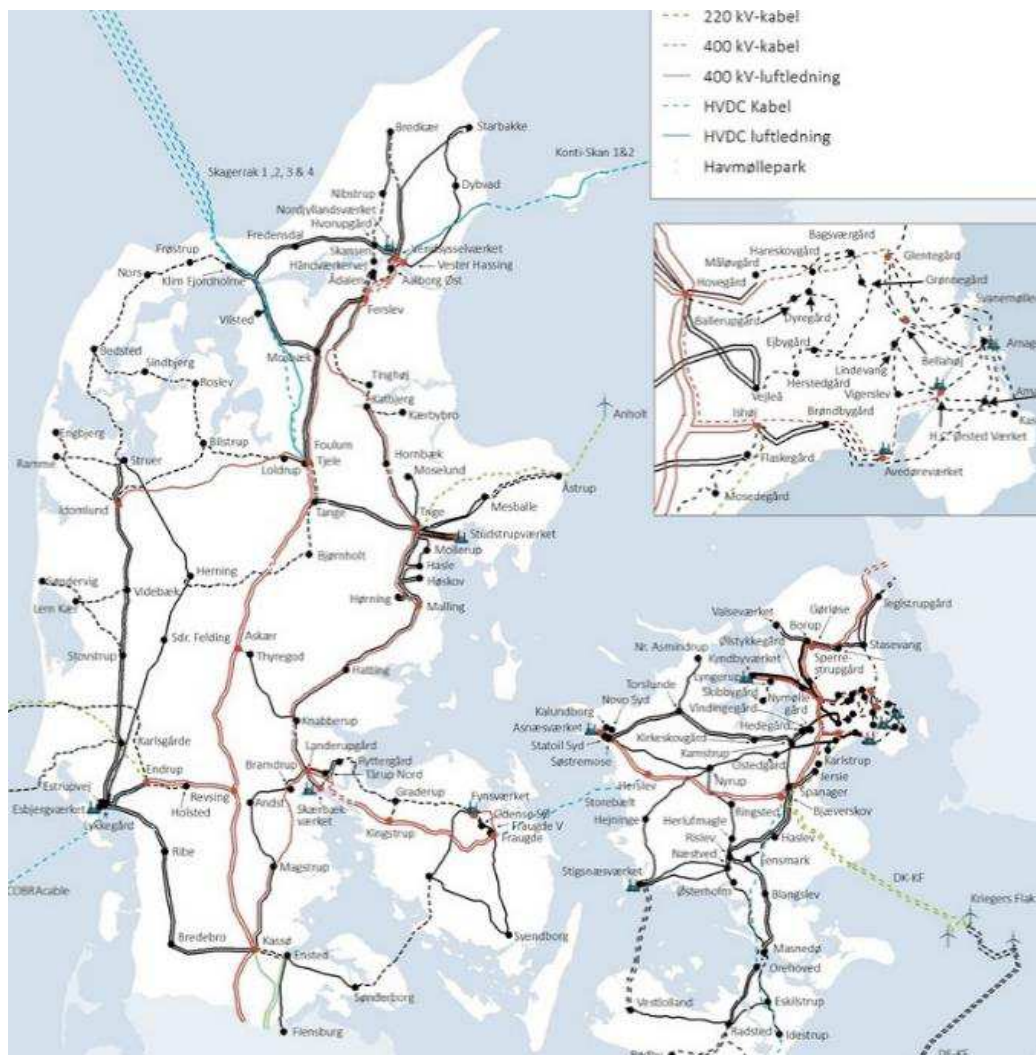
Figur 5 – Transmissionsstationer i Danmark
