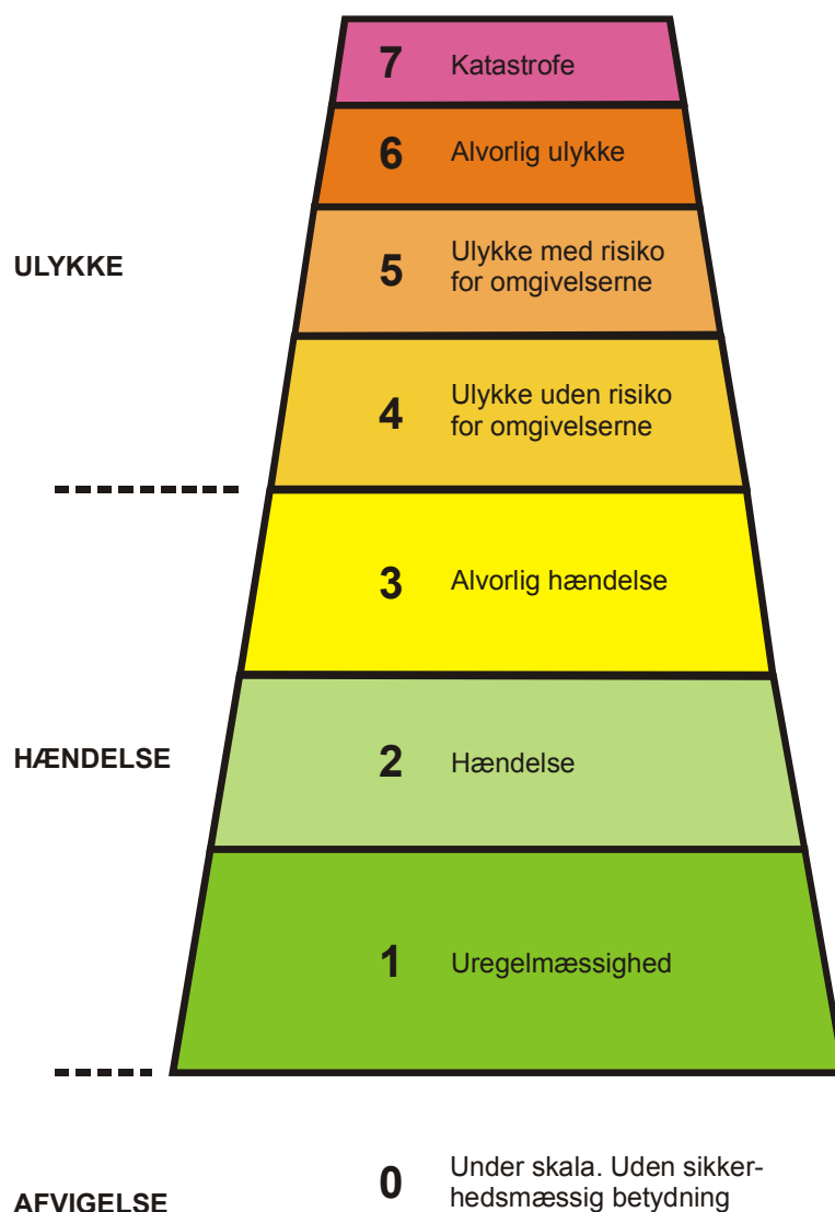
Figur 1 INES skalaen
