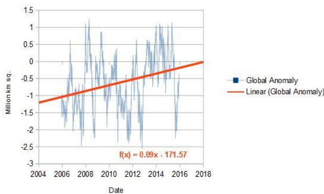
Global Sea Ice Area Anomaly
